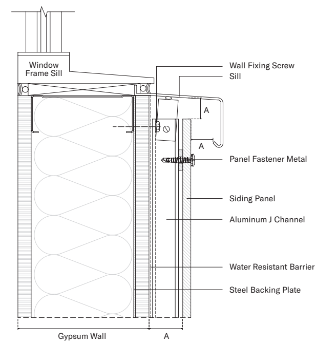
WINDOW SILL
