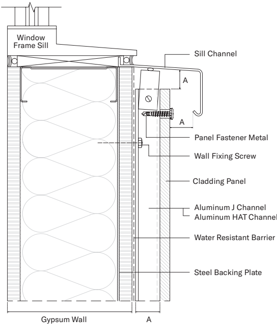
WINDOW SILL
