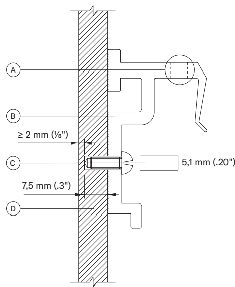
A. Machined M8 hole B. Fixing bracket C. Milling screw D. Cladding Panel
