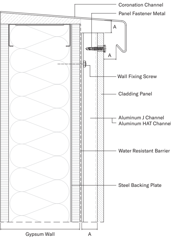
HEAD DETAIL
