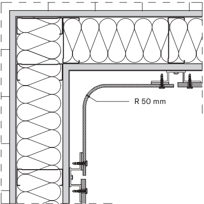
INTERIOR PRE-CURVED CORNER
