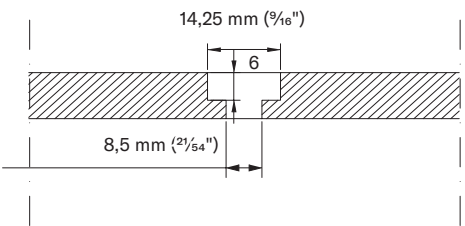
Fixed point
