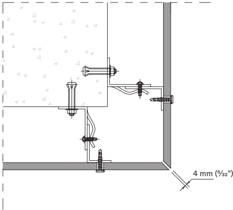
MITERED CORNER
