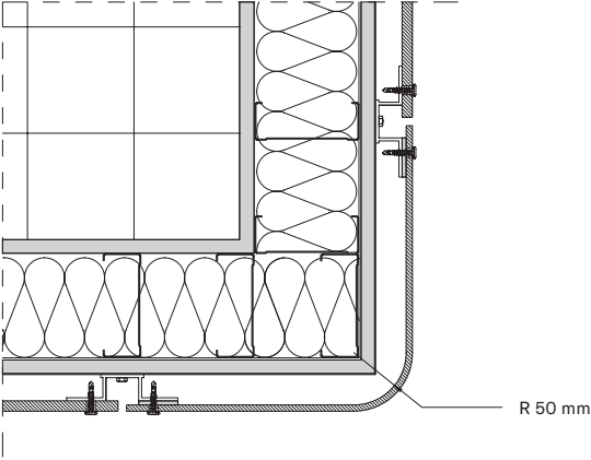
EXTERIOR PRE-CURVED CORNER
