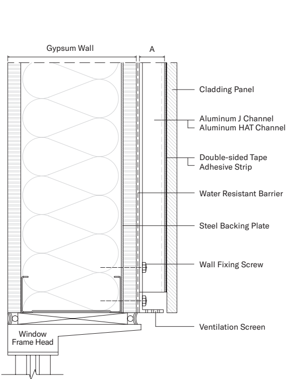
WINDOW HEAD
