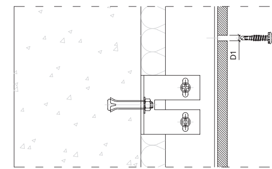
[ Fixed point ]
