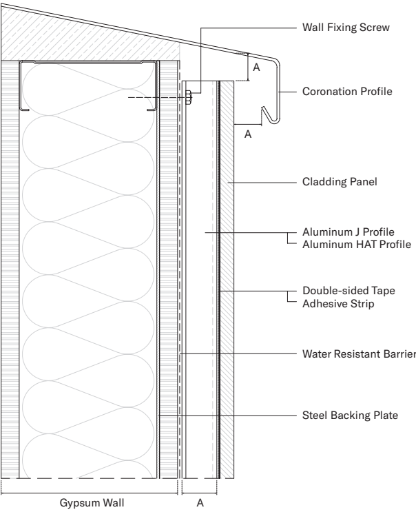
HEAD DETAIL
