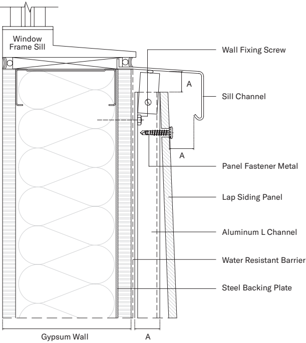
WINDOW SILL
