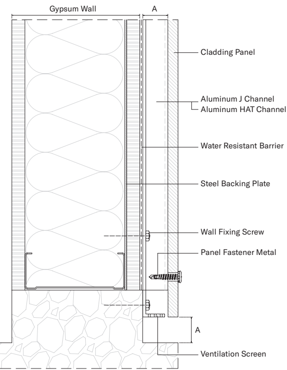
BASE DETAIL
