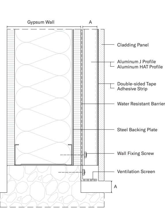
BASE DETAIL
