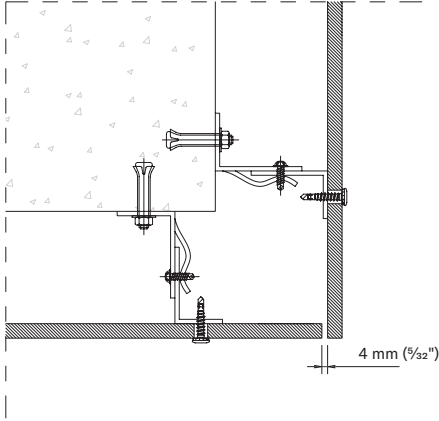
OVERLAPPING EDGE
