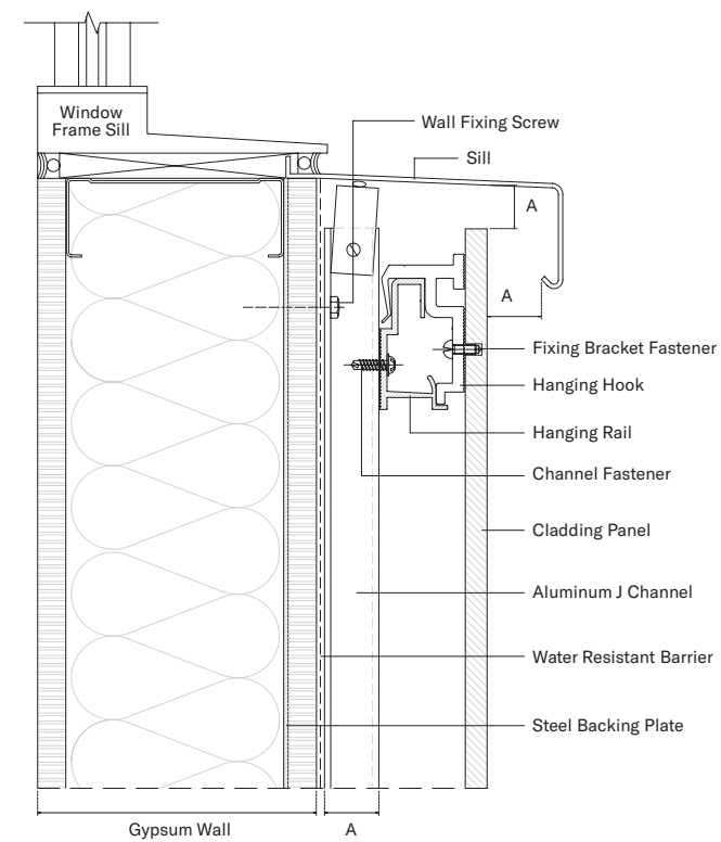
WINDOW SILL
