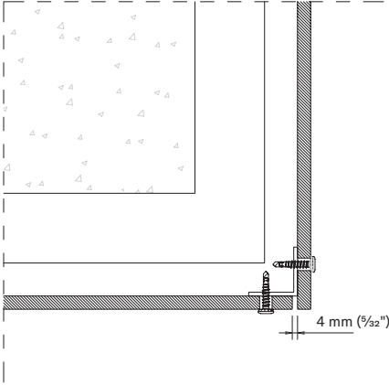
OVERLAPPING EDGE WITH REINFORCED CORNERS
