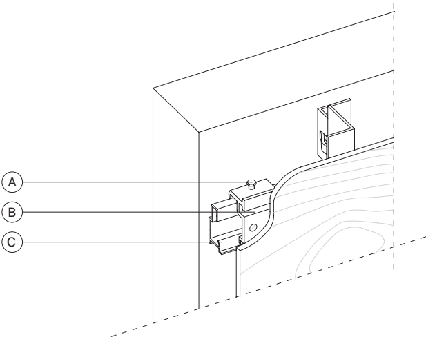
A. Height adjustment screw B. Panel fixing bracket C. Horizontal carrier rail
