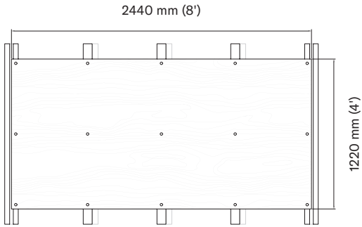
Profile distribution for 8-10 mm (5/16\"/>
