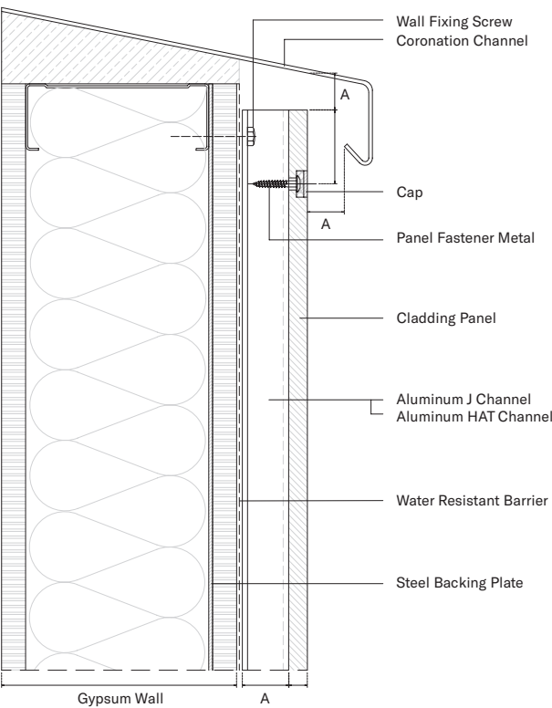
HEAD DETAIL
