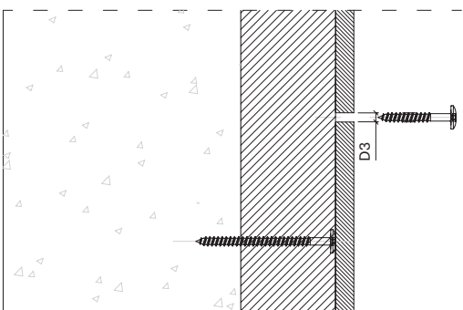
[ Fixed point ]
