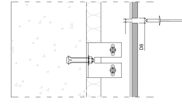
[ Fixed point ]
