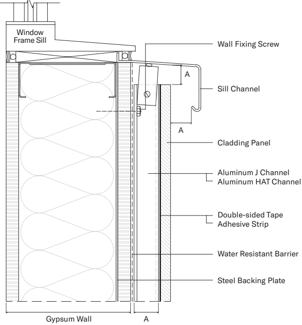
WINDOW SILL
