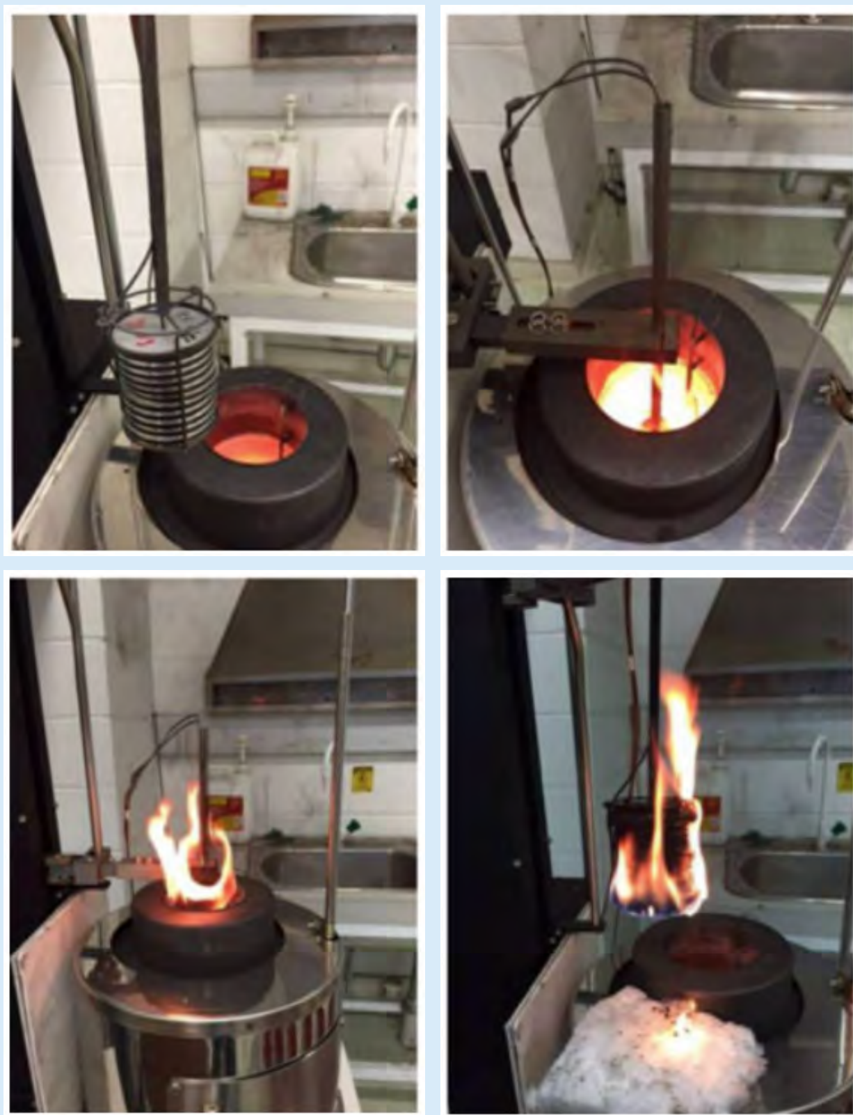
Figure 5.3: Fire test to AS 1530.1 (Source: ISpecify)
