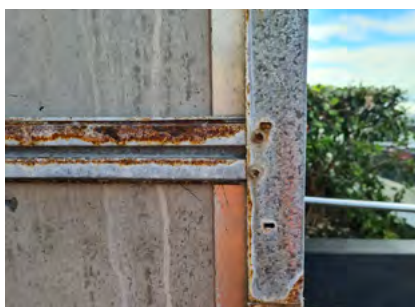
Figure 15.3: Standard galvanized coatings showing significant deterioration (located within close proximity to the coastline)
