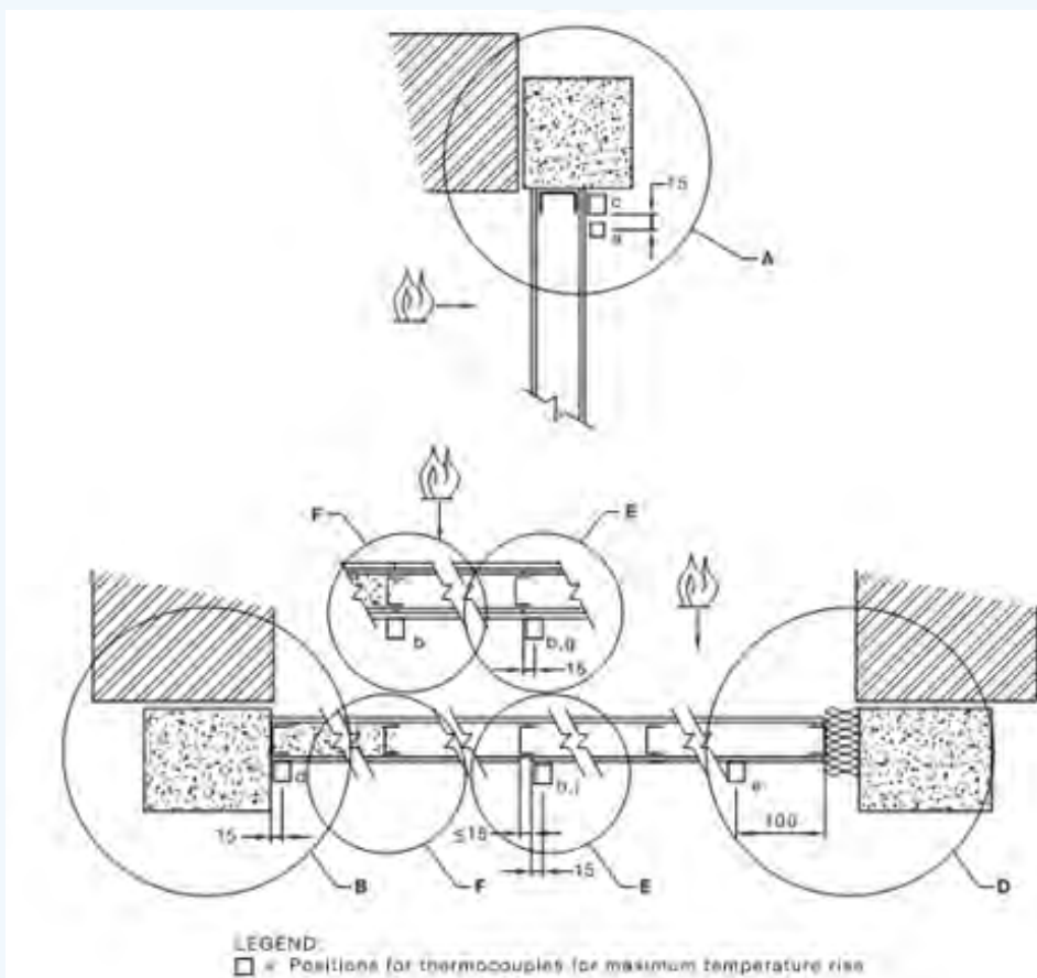
Figure 5.15: Typical configuration of thermocouples – Metal framework w/ horizontal linings (AS 1530.4)
